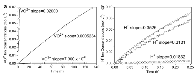
Figure 3. a) VO 2+ concentration and b) H + concentration versus time at the diffusion side of a diffusion cell using substrate, Nafion 115 and zeolite-coated membranes. Key: substrate (—Δ—), zeolite-coated membrane (—□—), Nafion 115 membrane (—○—).
